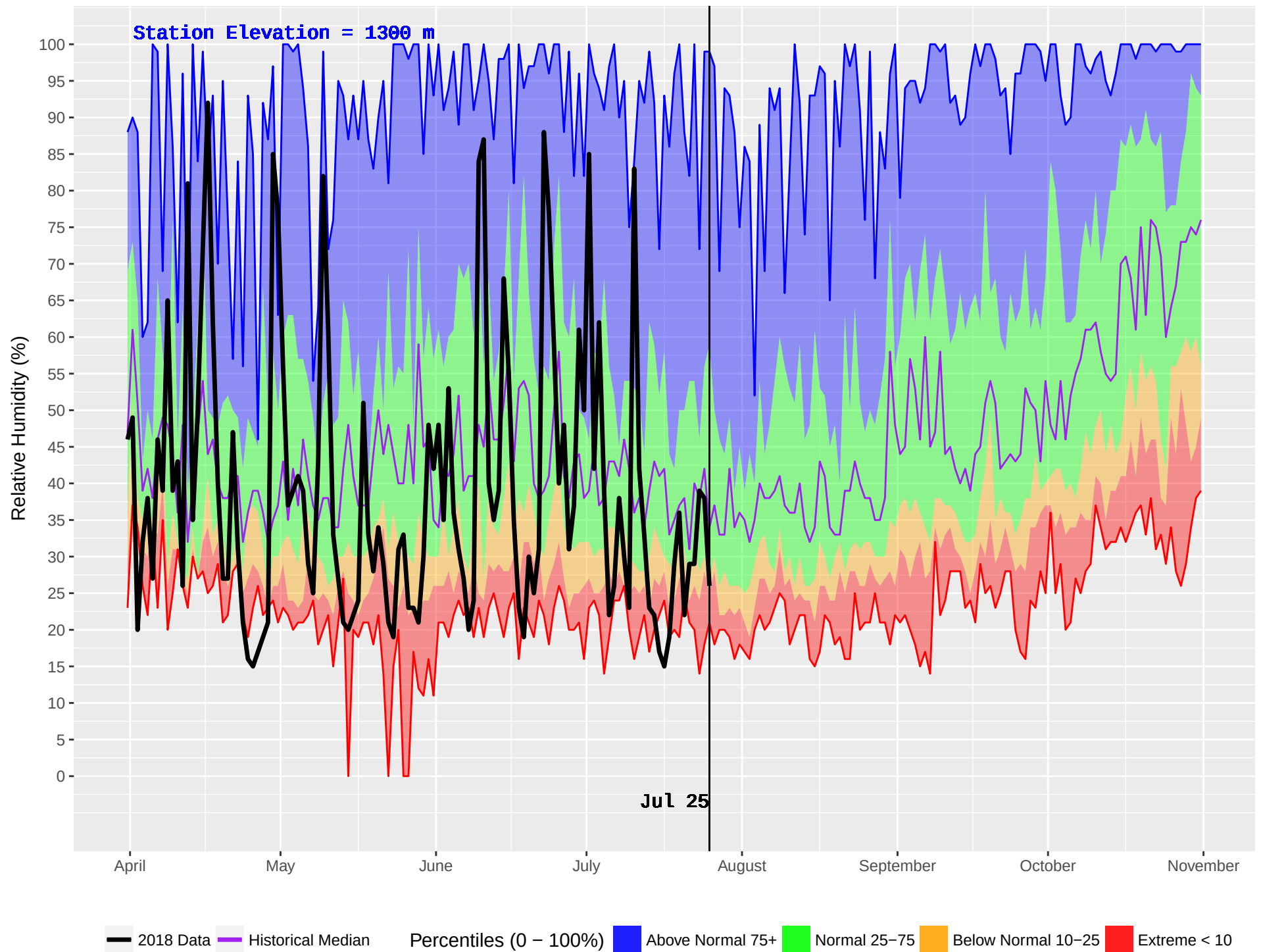
MARION (367) : Historical (1994–2016) and Current (2018) Noon Relative Humidity
