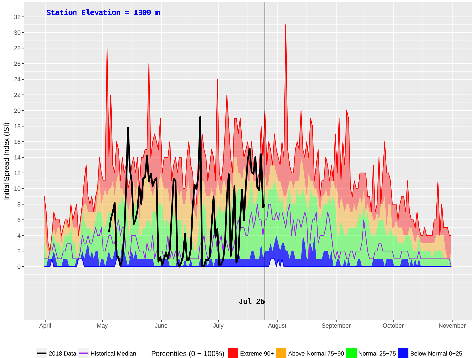
MARION (367) : Historical (1994–2016) and Current (2018) Noon Initial Spread Index (ISI)
